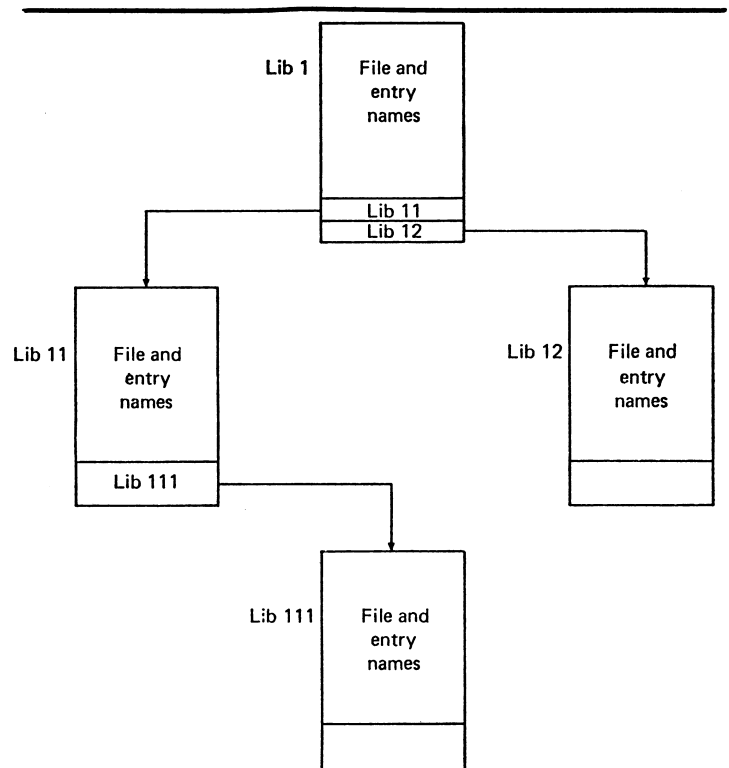
Fig. 5 Typical library index structure
