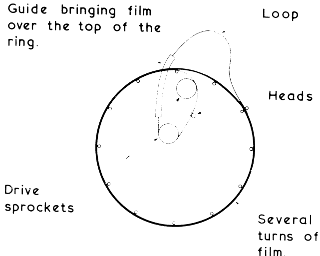
Fig. 1.—Principle of magnetic-film mechanism
